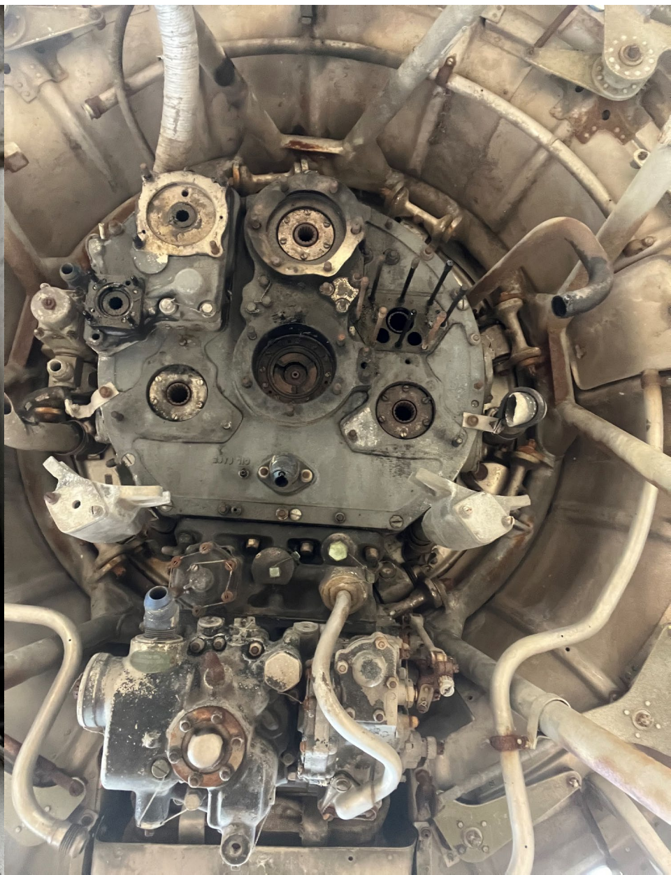
Removed from Northrop YC-125B aircraft: Engine, Wright R-1820-202A, MFRS. NO. 94373 (and propeller assembly)
