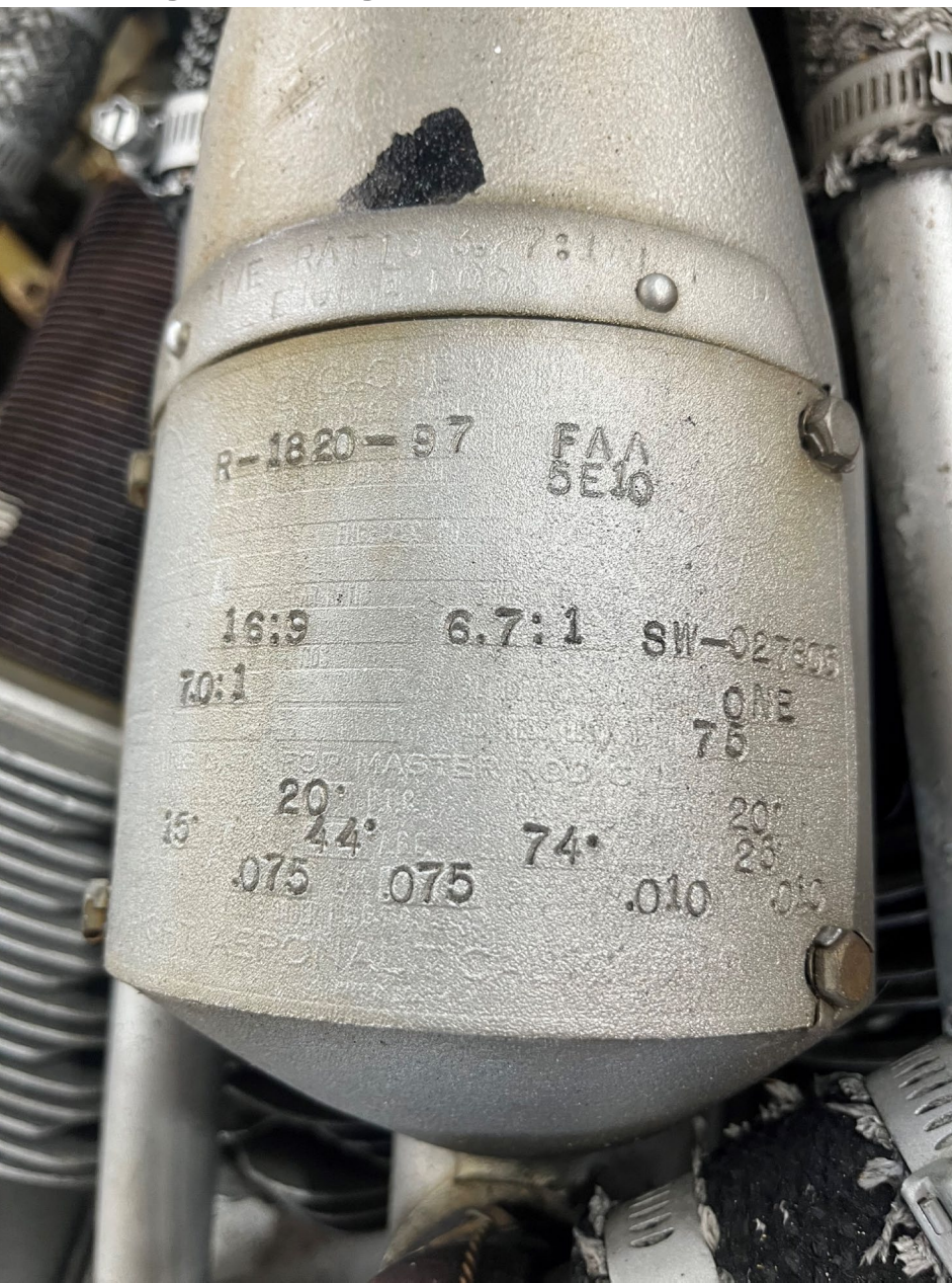
Removed from Northrop YC-125B aircraft: Engine Wright R-1820-97, MFRS. NO. SW-027805 (and propeller assembly)
